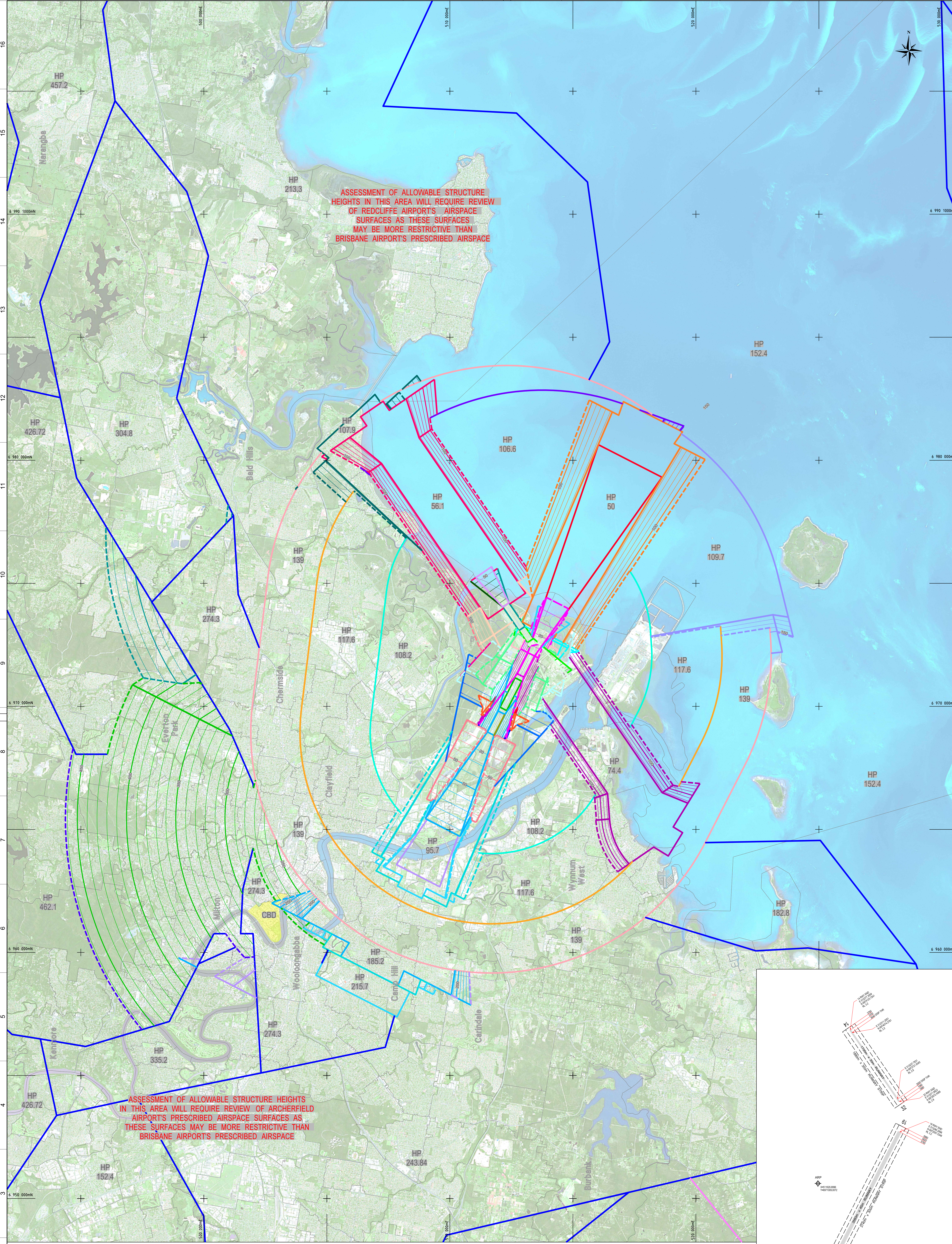
PANS-OPS surfaces procedures Existing development
